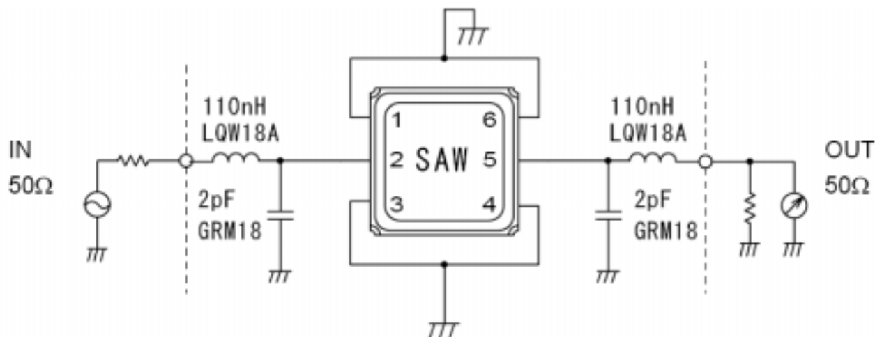
Fig.1 Measuring circuit
